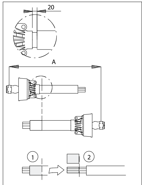
Fig. 2. Shorten the drive shaft
